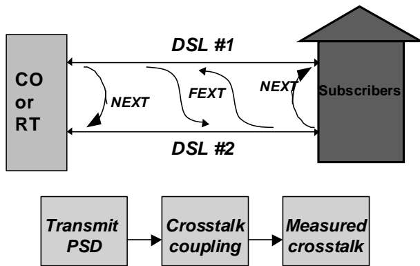
Figure 4. Crosstalk: transmitted signal, coupling, and received crosstalk
